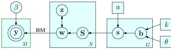
Fig. 2. The graphical model of linear regression with hierarchical priors. \mathbf{y} and \mathbf{z} are Gaussian distributions, \mathbf{w} is a GSM, \mathbf{s} and \mathbf{b} are Gamma distributions.
