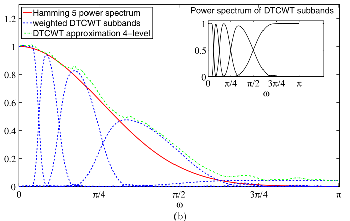
Fig. 11. Weighted power spectrum of 1-D DT CWT subbands, (a) selection of \alpha_j using (59), (b) \alpha_j are increased to account for energy leakage.
