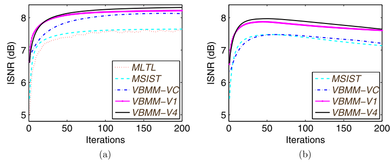
Fig. 6. ISNR results using (a) analysis algorithm (b) synthesis algorithm, on Cameraman, 9 \times 9 uniform blur, BSNR = 40 dB.
