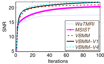
Fig. 10. SNR results for CS MRI reconstruction over 100 iterations, on Chest image.
