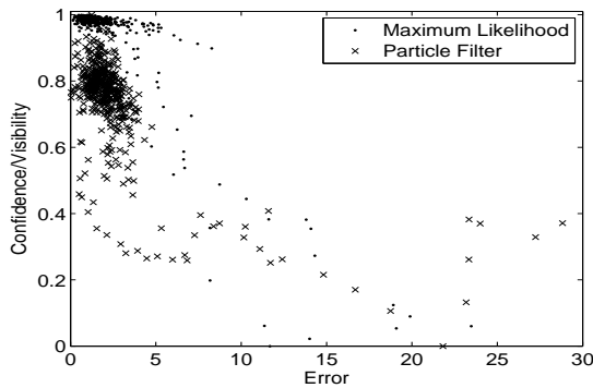
Figure 7. Scatter plot of error against confidence/visibility for the maximum likelihood and particle filter methods.
