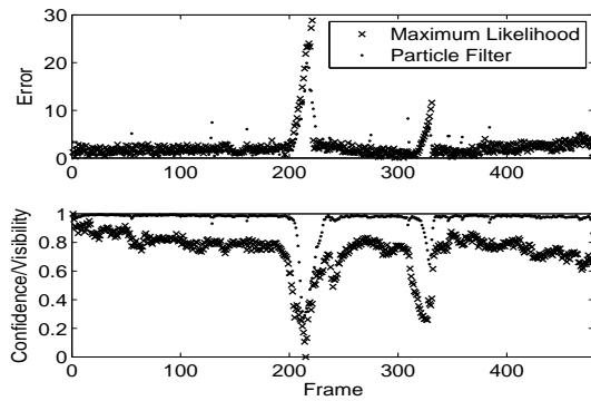
Figure 6. Error and confidence/visibility for the maximum likelihood and particle filter methods for each frame in the image sequence. The two methods result in similar performance. The spikes in the particle filter method occur as the posterior distribution stretches or splits into two modes to account for uncertainty in the position of the target. However, the particle filter does seem to be more reliable in the event of total occlusion by smoke, around frame 210, and partial occlusion by buildings, around frame 320.
