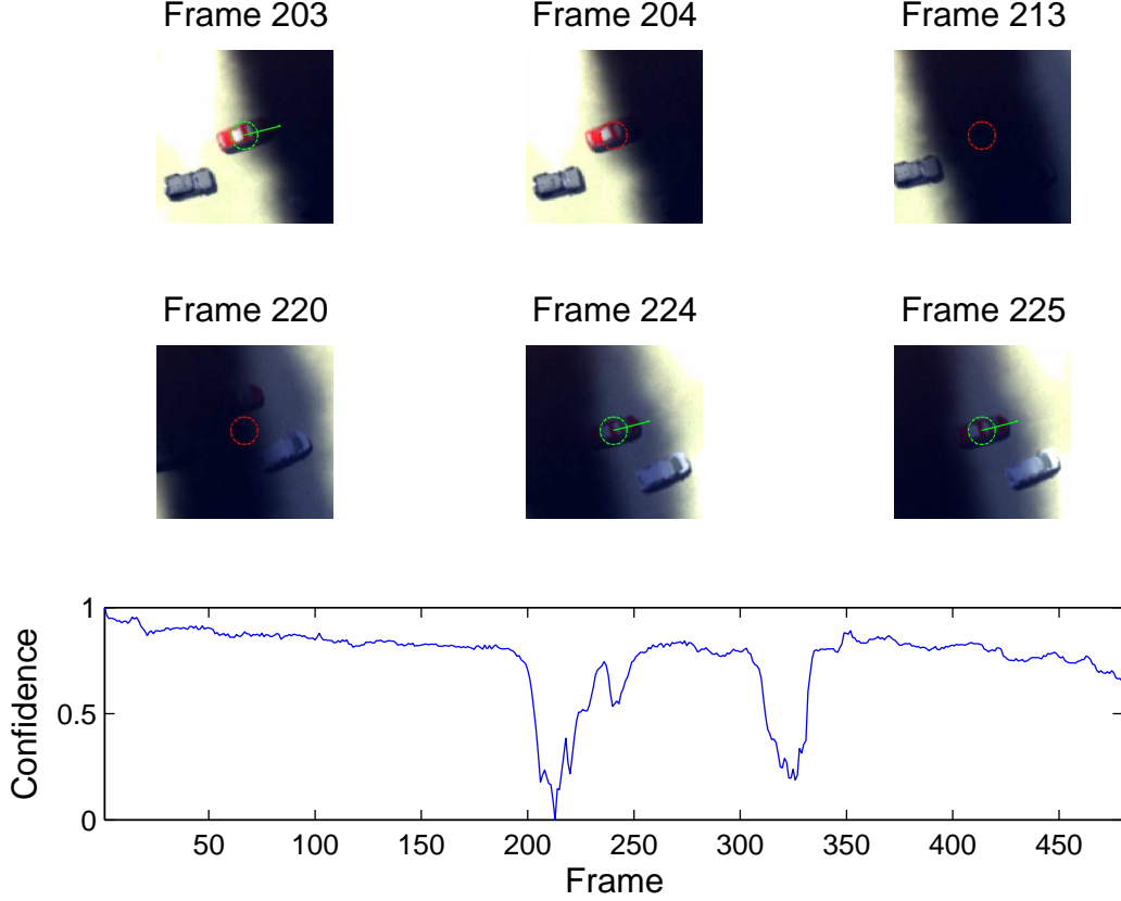
Figure 4. Frame 203: Correlation score close to decreasing below threshold value; 204: threshold breached, search window extended, and extrapolation invoked; 213: full occlusion; 220: score increases and approaches threshold; 224: score becomes greater than threshold and target is reacquire; 225 window narrows and extrapolation terminated.
