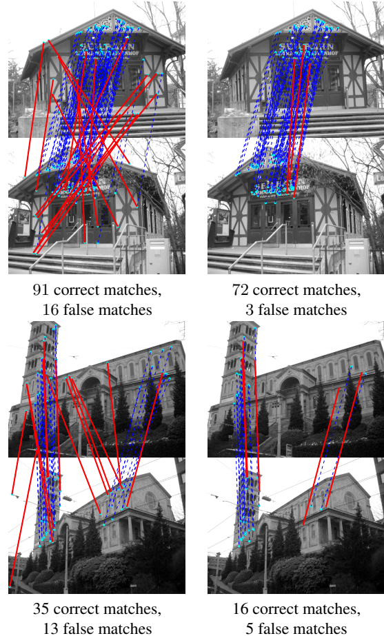
Fig. 3: Matching results for a pair of complex scene. False matches (red) can be observed for both the proposed algorithm (right) and baseline SIFT (left), however the proposed algorithm produces much fewer false matches, thus resulting in more robust matches.
