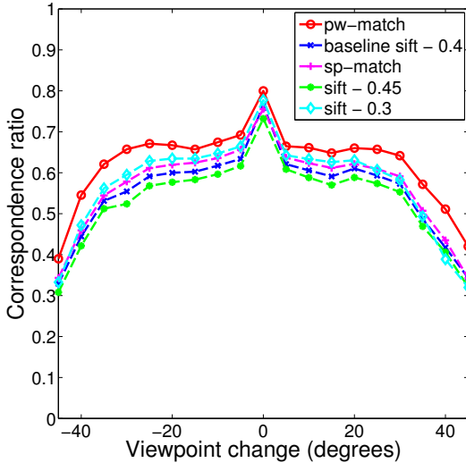
Fig. 2: Correspondence ratio for viewpoint changes. The proposed algorithm pw-match has a higher ratio compared to the algorithms tested. The improvement is more significant at larger viewpoints, suggesting that spatial constraints can be used to produce more robust matches. Similarly, pw-match has a higher ratio as the distance ratio threshold is varied for baseline SIFT.
