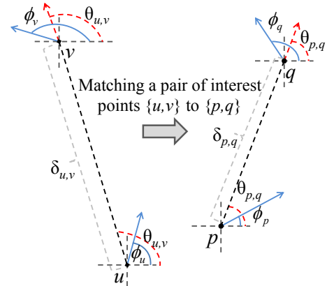
Fig. 1: Matching a pair of interest points u, v to a second pair p, q . \theta_{u,v} is the direction of the vector between u, v and \delta_{u,v} is the distance between u, v (similarly for \theta_{p,q} and \delta_{p,q} ). \phi_u, \phi_v, \phi_p, \phi_q are feature orientations at interest points u, v, p, q .
